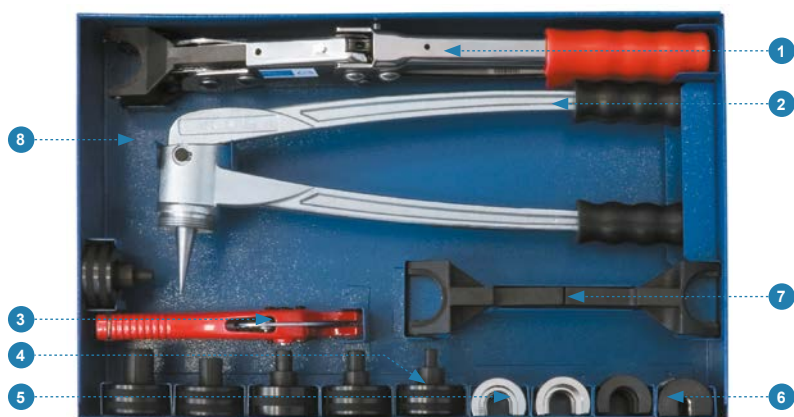
Rys. 2 Case set for hand chain press
